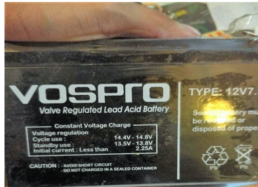
Figure 2 Battery
