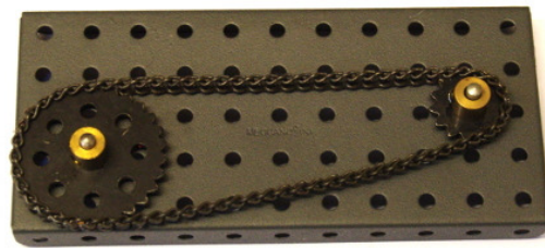
Figure 3 Chain Drive
