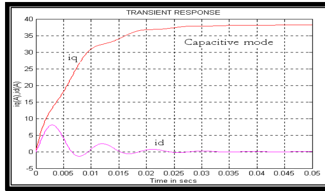
Figure 8 Transient response of i_d and i_q in capacitive mode
