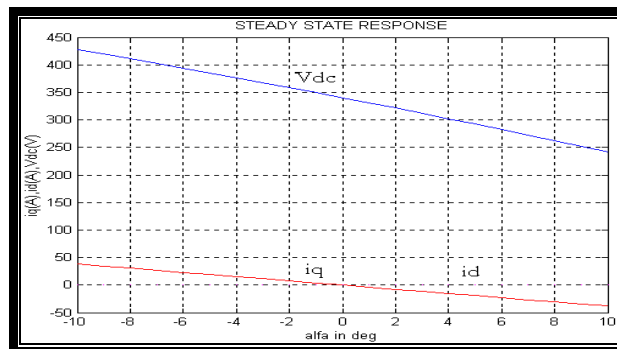
Figure 7 Steady state response of i_d and i_q
