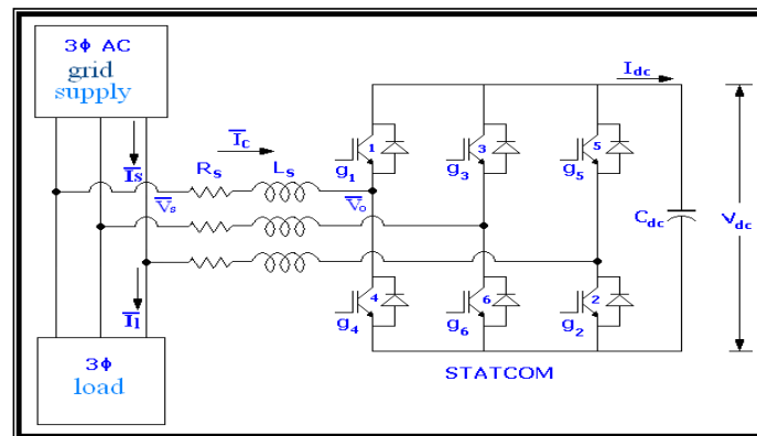
Figure 1 Configuration of STATCOM
