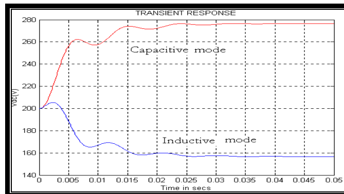
Figure 10 Transient response of v_{dc} in both modes
