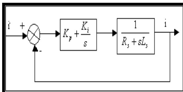
Figure 5 Effective closed loop current control system
