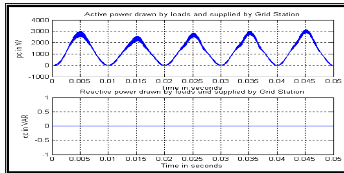
Figure 16 Grid supplied active and reactive power to R-L load after operation of the STATCOM
