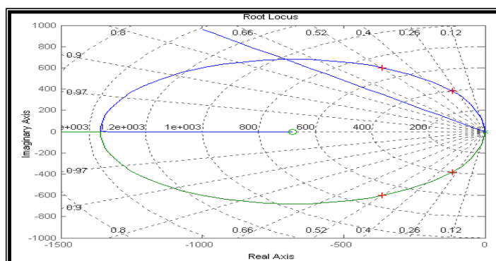
Figure 4 Root locus plot
