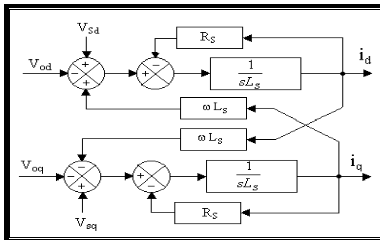
Figure 2 Equivalent Diagram on a.c. side of STATCOM
