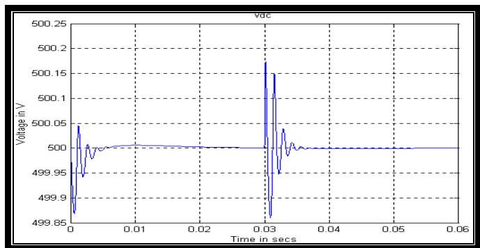
Figure 12 Voltage Control with reference
