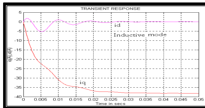
Figure 9 Transient response of i_d and i_q in inductive mode
