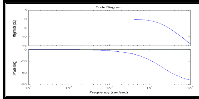
Figure 6 Bode plot of the system with PI
