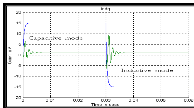
Figure 11 Current control with reference
