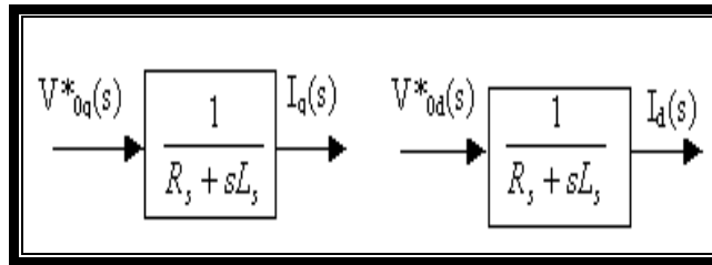
Figure 3 Current control of inverter of equivalent decoupled SISO systems
