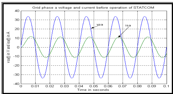
Figure 13 Grid phase-a voltage and current with R-L load before operation of the STATCOM
