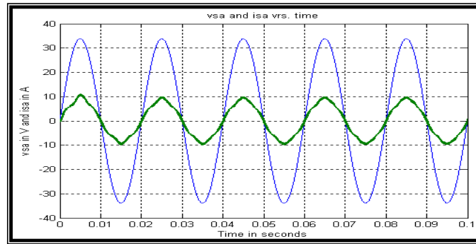
Figure 15 Grid phase-a voltage and current with R-L load after operation of the STATCOM
