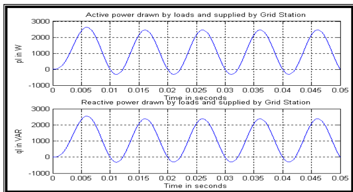
Figure 14 Grid supplied active and reactive power to R-L load before operation of the STATCOM
