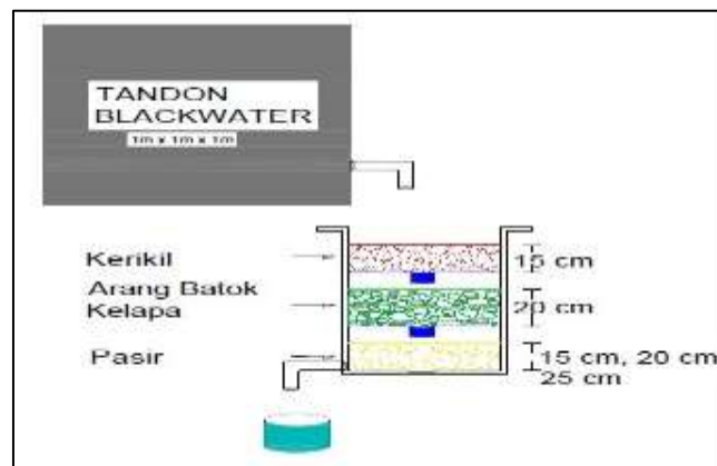
Figure 1 Filter materials (Gravel 12,5 mm, Charcoal 2 mm and Sand 2 mm)
