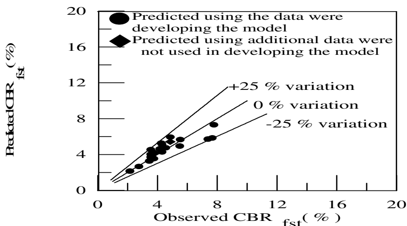
Figure 7 Predicted CBR_{fst} versus observed CBR_{fst} curve
