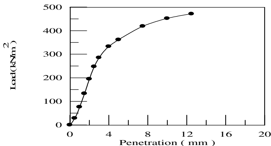
Figure 4 Typical load versus penetration curve for subgrade soil of JBD roads (September,2014)
