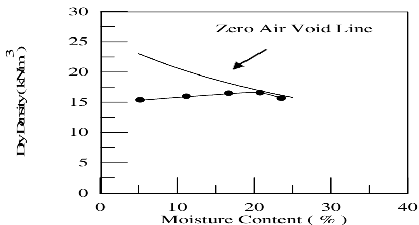
Figure 2 Typical dry densities versus moisture content curve for subgrade soil of JNH road
