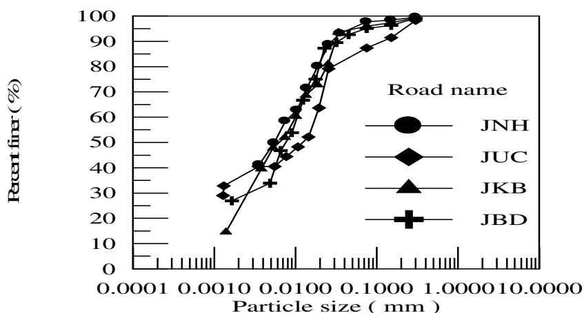
Figure1 Grain size distribution curve for subgrade soil for four different
