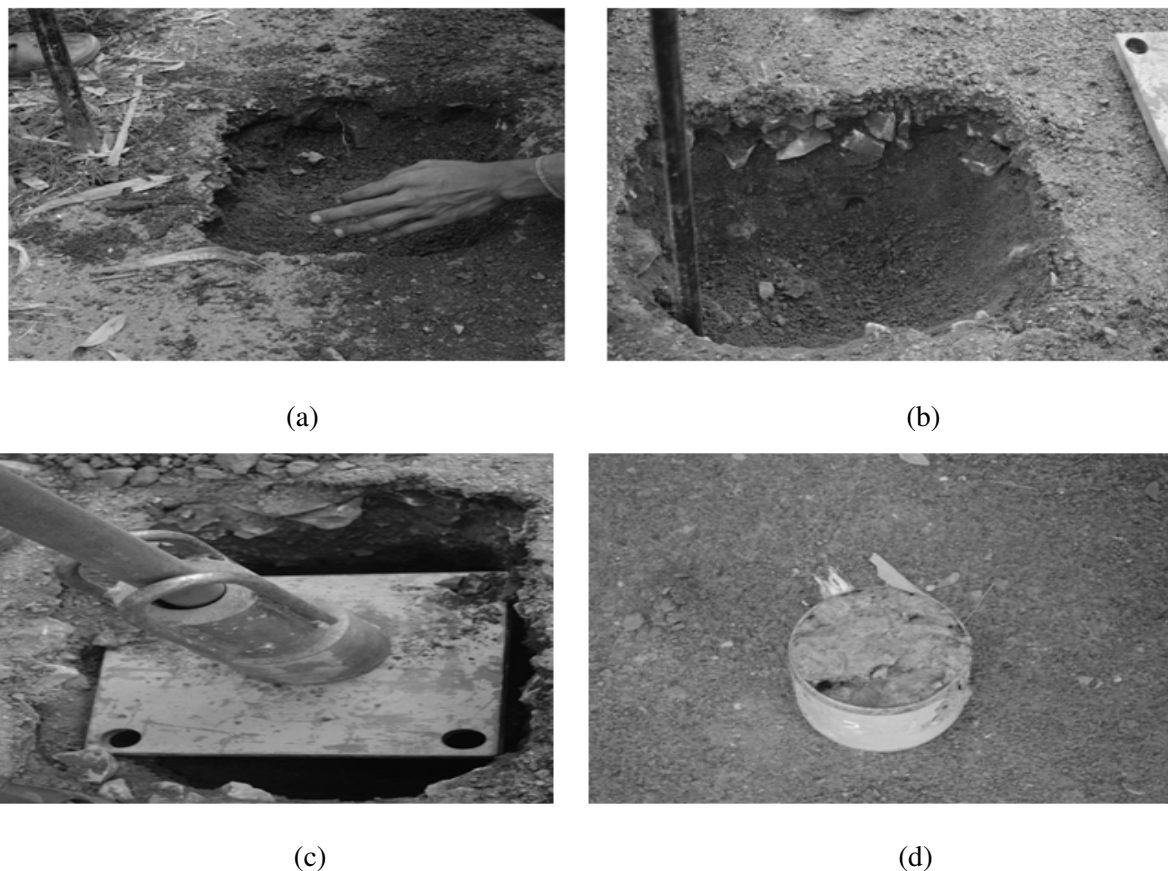
Figure 3 Photo plates during collection of CBR sample of JBD road. ( a ) Marking for the excavation of pit; ( b ) Excavation is in progress; ( c ) Penetration of CBR mould into subgrade soil with the help of Hammer and plate; ( d ) CBR sample from field (before dressing).
