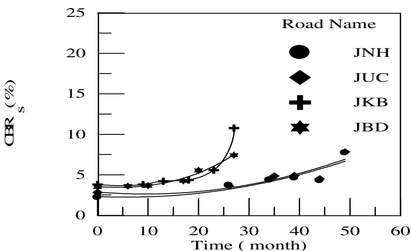
Figure 5 CBR us versus time curve for different roads
